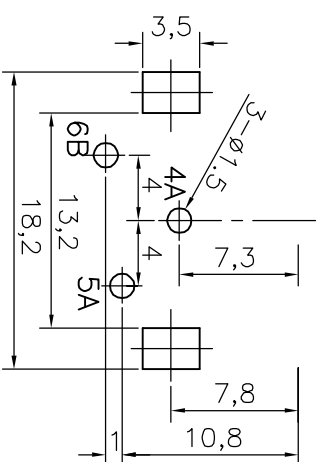
P.C.B. HOLE LAYOUT (BOTTOM VIEW)
